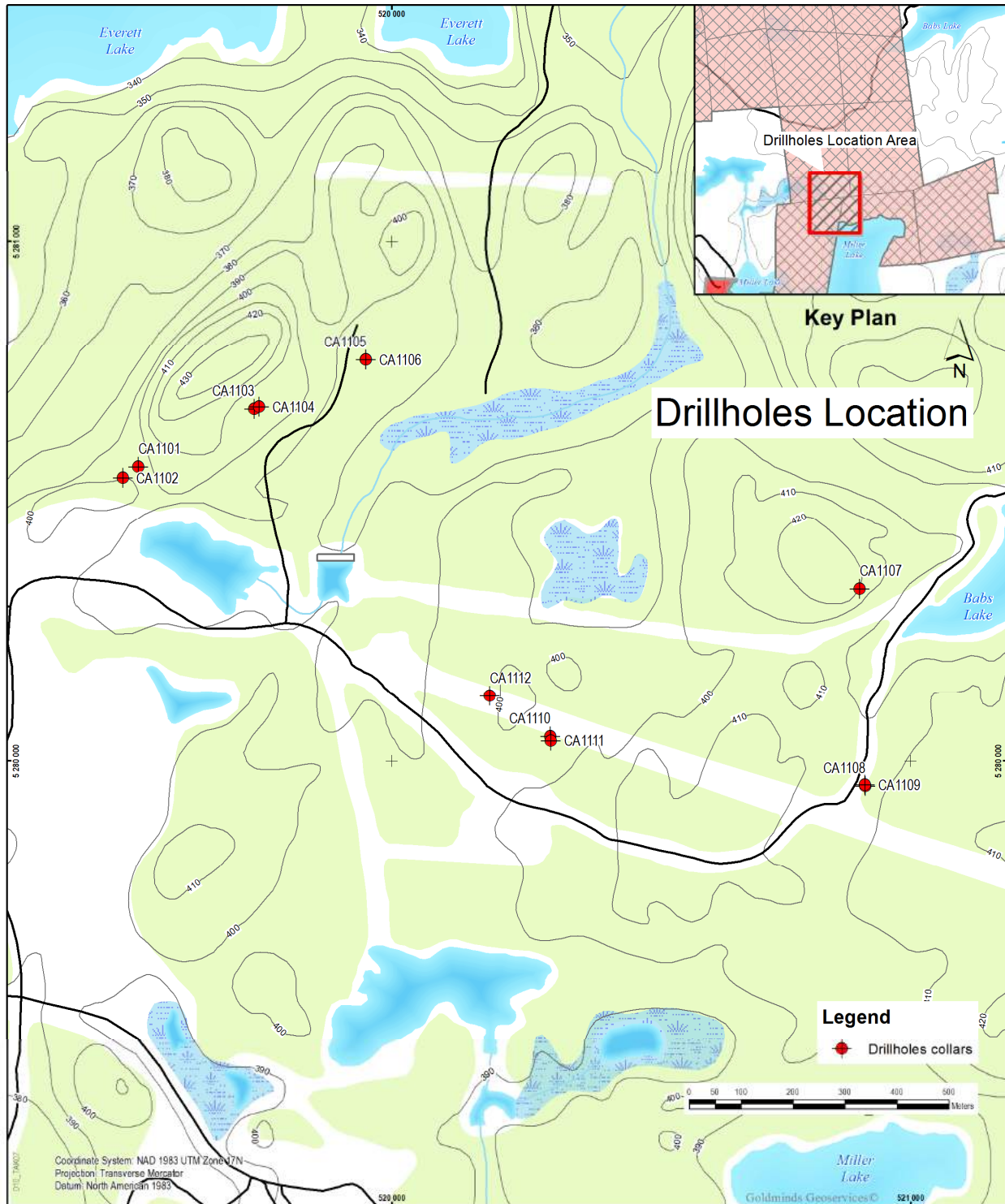
Figure 30 : Location of the Diamond Drill Collars
