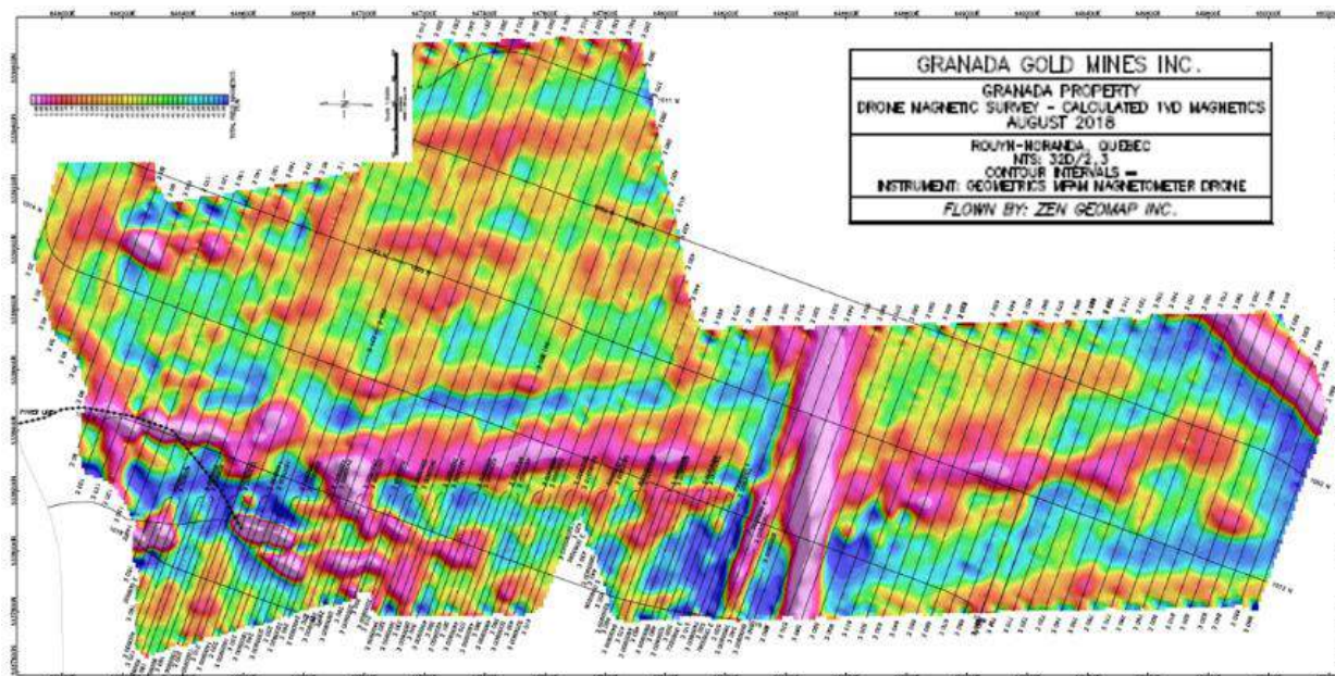
Figure 9-5 Drone- Magnetic Survey calculated 1VD Magnetics, Granada
