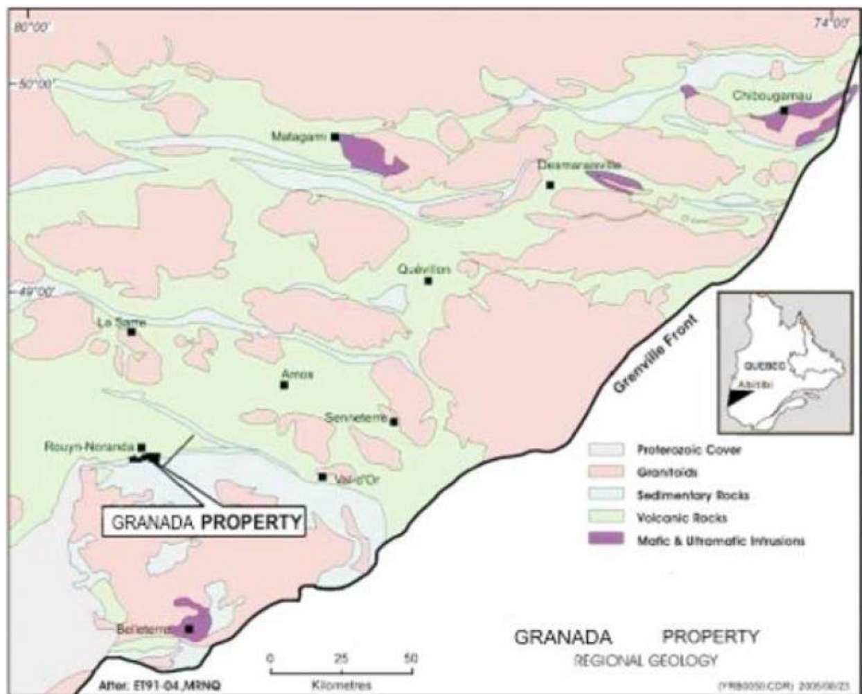
Figure 7-2 Regional Geology
